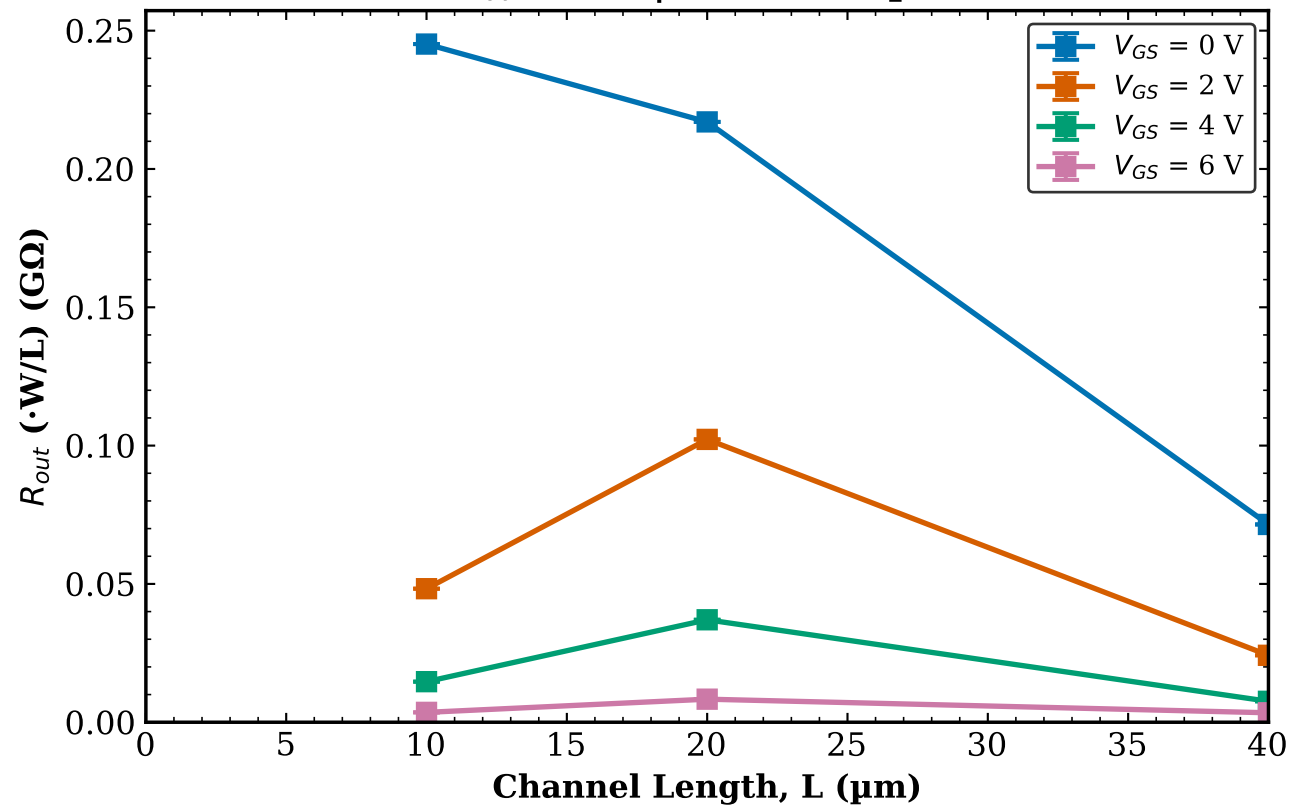
TFT3 Transistor 1 R_{out} vs L | W = 100\text{ }\mu\text{m}
